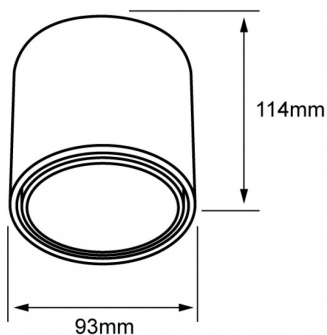
Downlights 12 W
