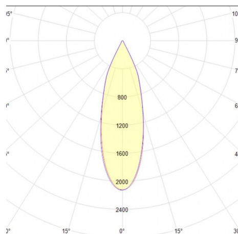
Downlights 12 W / 34°
