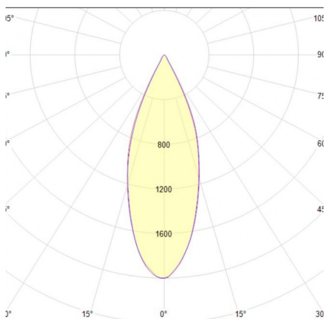
Downlights 15W / 37°
