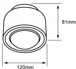
Downlights 15W
