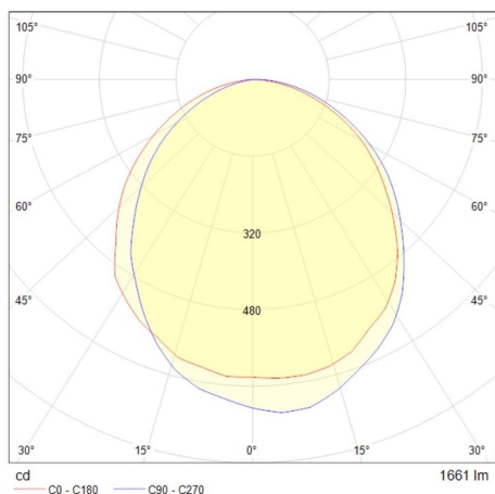
Ultralim 18W
