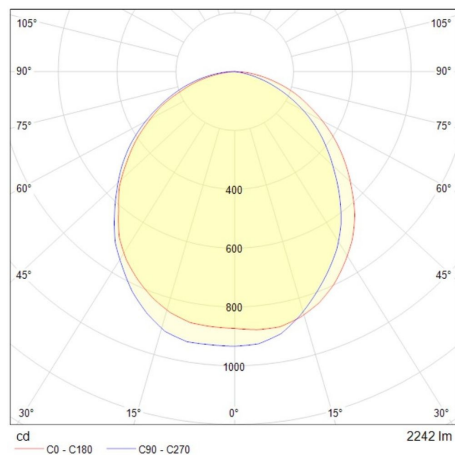
Ultralim 24W
