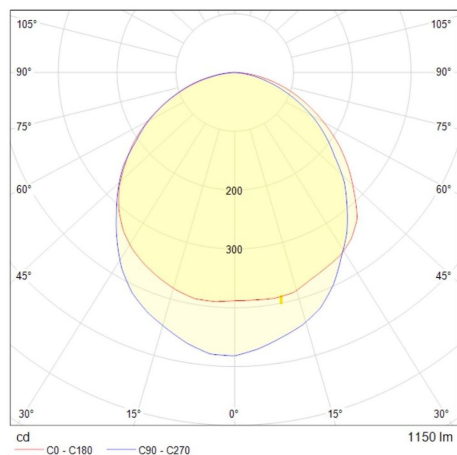
Ultralim 12W
