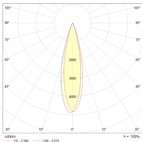
Focus 30W 24°
