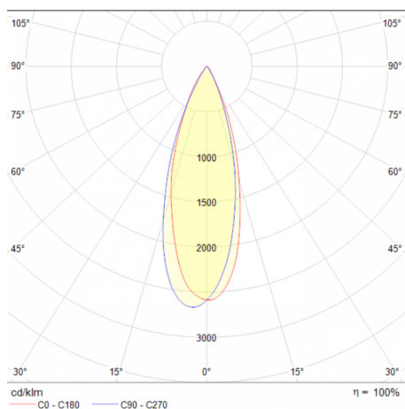
Focus 45W 36°
