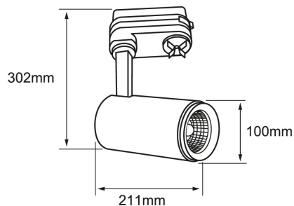
Focus 30W
