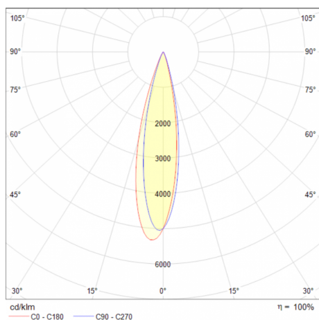
Focus 45W 24°
