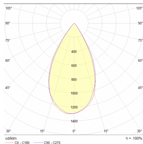
Focus 45W 60°
