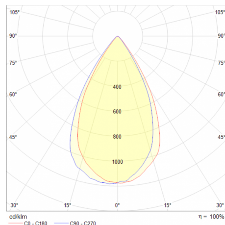
Focus 30W 60°
