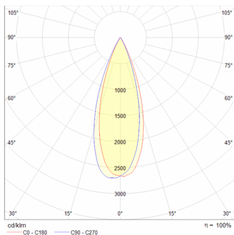
Focus 30W 36°
