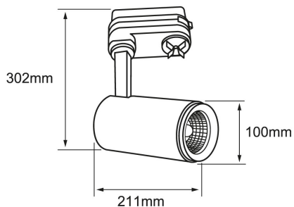
Focus 45W
