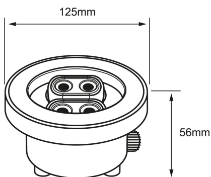
Uplight 10W Redondo
