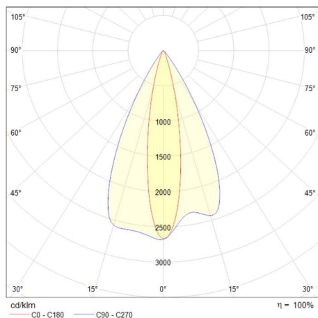
Uplight 20W Redondo
