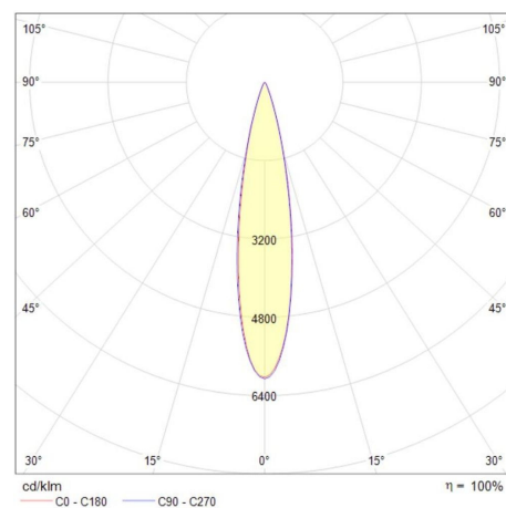
Uplight 13.5W Redondo
