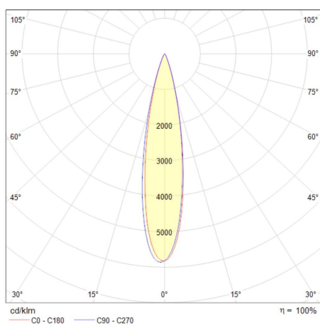
Uplight 10W Redondo
