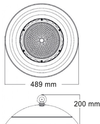
Highbay Pure 200W
