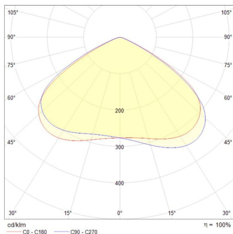
Highbay Pure 150W
