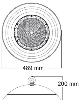
Highbay Pure 150W
