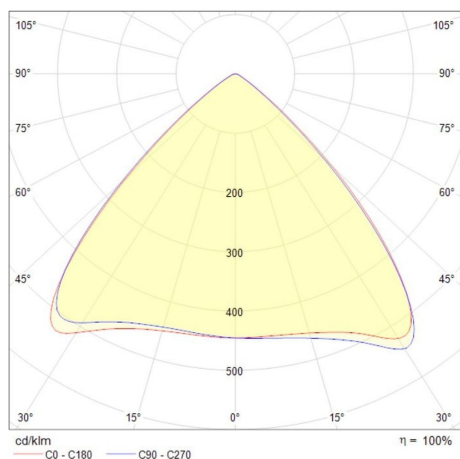
Highbay Pure 100W
