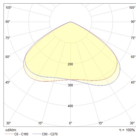
Highbay Pure 200W
