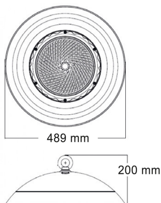
Highbay Pure 100W
